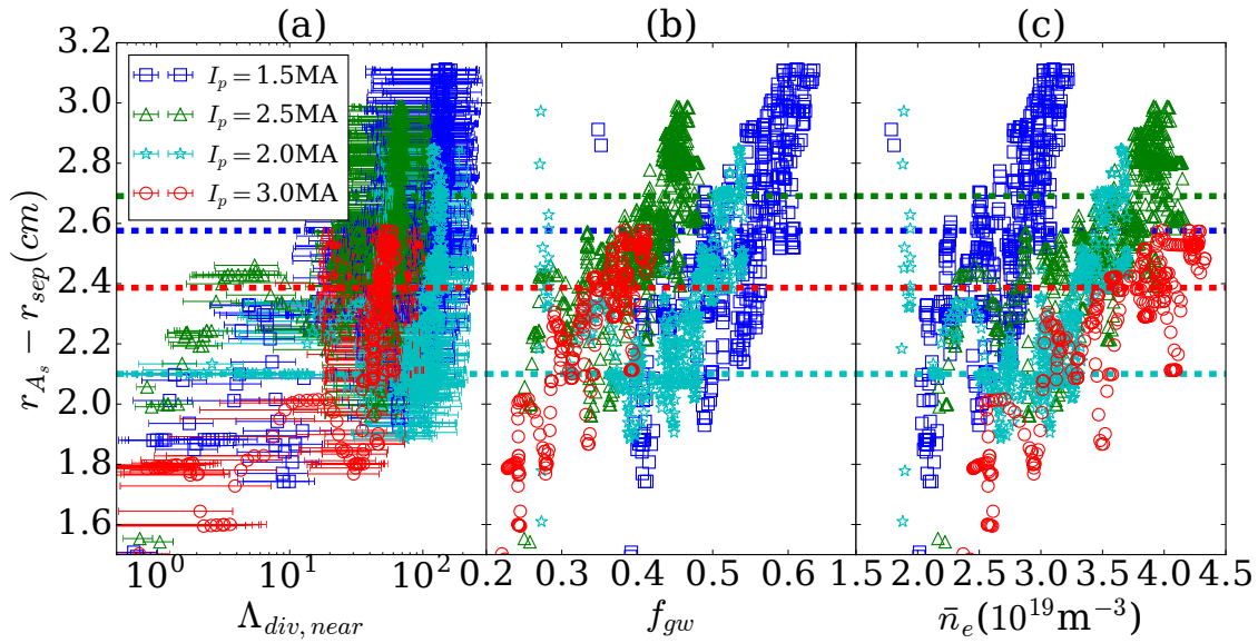
Figure 8: Movement of the radial location of A_s as a function of \Lambda_{div} (a), \bar{n}_e/n_{gw} (b) and \bar{n}_e (c) for the 4 plasma currents of Fig. Ip_scan with L-mode, horizontal target plasmas and D 2 puffing driving a core density ramp. (a) Indicates the 2 phases of the profile evolution, initially formation and subsequent growth. Horizontal lines indicate the onset of detachment for each plasma current.
