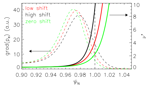
Figure 13. Electron pressure gradient (dashed lines) and effective collisionality (full lines) comparison for low ( 1\%\psi_N , red color), high ( 3\%\psi_N , black color), and zero pedestal relative shift (green color). Vertical black dashed line represents the separatrix.
