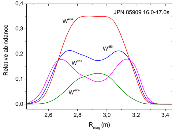
FIG. 5. Fractional abundance for W^{44+} - W^{47+} tungsten ions calculated for JET shot #85909 (time 16.0-17.0s).
