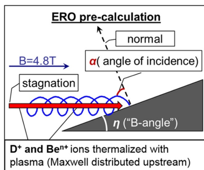
Fig 4. Model situation considered for generation of the energy E_{in} and angle \alpha distributions on the ion impact with the surface inclined by the angle \eta with the B-field ( \sim 4.8 T at ITER B11 location).
