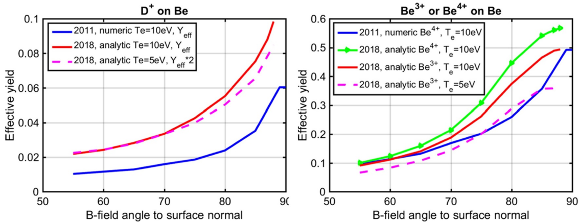
Fig 5. The effective sputtering yields for Be by D + ions (left) and Be ions (right) simulated using the semi-analytical sheath approach [10] and pure numerical procedure used in 2011. T e = 5 eV curve for D + impact (left) is multiplied by 2 to simplify the shape comparison with the T e = 10 eV.
