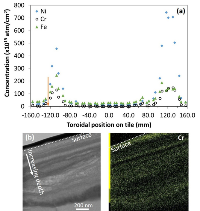
Fig. 3. (a) Nickel, chromium and iron concentrations on mid-plane inner wall guard limiter tile after ILW3. (b) Transmission electron micrograph and elemental analysis showing layered deposit containing chromium from ILW1 Be limiter tile. The arrow in (a) indicates the toroidal location of the micrographs. Also indicated by a cross in Fig. 4.
