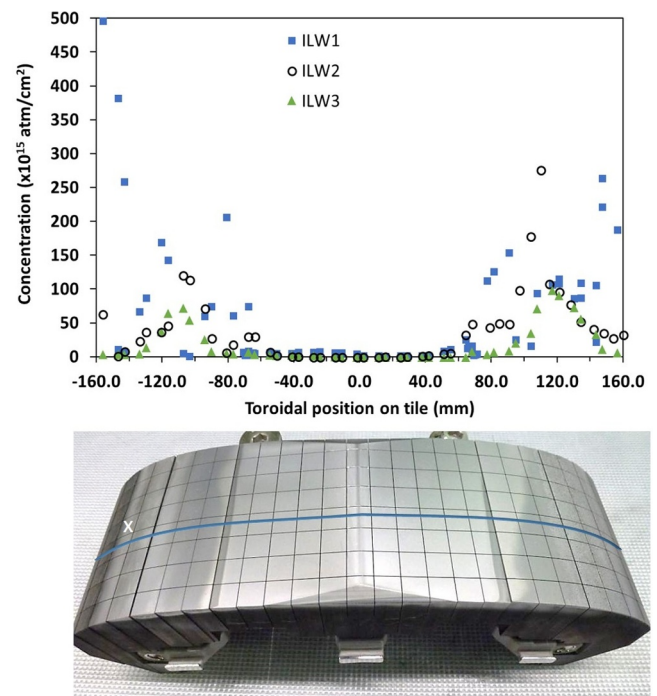
Fig. 4. Tungsten concentration on tiles located at the mid-plane of the IWGL after each ILW campaign. The line on the tile photograph indicates the analysis line toroidally across the tile. The cross on the left of the tile photograph indicates the location of the micrographs shown in Fig. 3.
