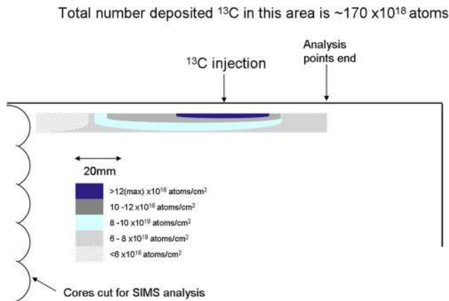
Fig. 56. A 2-dimensional plot of the ^{13}\text{C} deposit of a Tile 7 (2ONG7A) as derived from RBS spectra, in the region adjacent to a gas injection nozzle between Tiles 7 and 8 at the top of the front surface. The maximum is in a region normally protected from incident ions by the slightly prominent lower edge of Tile 8. The ^{13}\text{C} flow is in the direction of the arrow beneath “ ^{13}\text{C} injection”.
