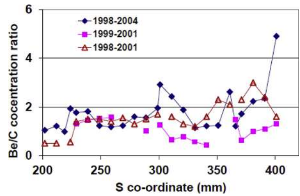
Fig. 31. Be/C ratios determined by NRA for Tile 1 - examples from different operational campaigns. The apron is between s-coordinates 162 and 222 mm and the front face of the tile from 222 to 431 mm.
