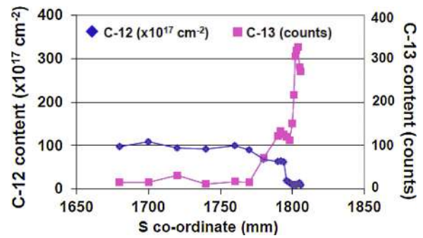
Fig. 57. Plot of ^{13}\text{C} and ^{12}\text{C} measured by NRA across Tile 2ONG7A, showing that the deposit at the top edge is almost exclusively ^{13}\text{C} and not ^{12}\text{C} .
