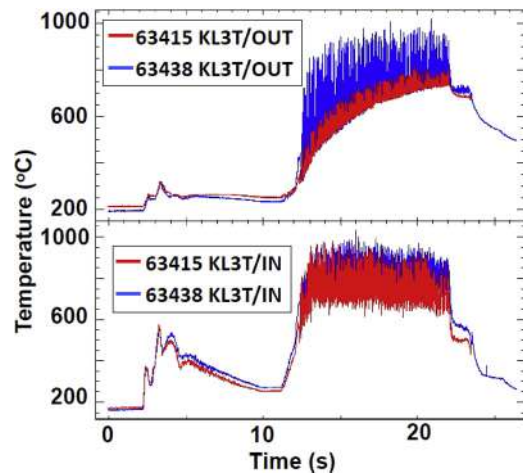
Fig. 58. Maximum temperatures measured with an infra-red camera during selected pulses during the ^{13}\text{C} puffing experiments at the end of the 2002–4 campaign. The upper part shows the maximum temperature in the outer divertor during pulse 63415 (red curve) and 63438 (blue curve). The lower part shows the maximum temperature in the inner divertor during pulse 63415 (red curve) and 63438 (blue curve) (For interpretation of the references to colour in this figure legend, the reader is referred to the web version of this article).
