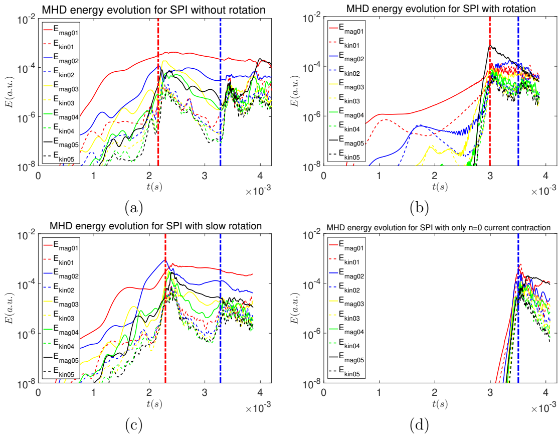
Figure 18. The comparison of the perturbed magnetic and kinetic energy of n = 1 - 5 modes for the JET-like SPI in (a) a stationary plasma, (b) a rigid body rotating plasma with rotation frequency 10kHz , (c) a rigid body rotating plasma with rotation frequency 1kHz and (d) a plasma where the n = 0 current contraction is the only MHD destabilizing mechanism. The red and blue chained lines indicate the onset time of the first and the second TQ.
