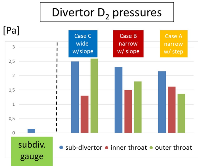
Fig. 7. Modelled molecular pressure p_{D2} at the inner and outer divertor louver regions (c.f. purple circles in Fig. 3), and at the location of the sub-divertor pressure gauge (red circle in Fig. 3). For comparison the experimental value for the sub-divertor pressure is shown too, showing a massive discrepancy (one order of magnitude) to the modelled p_{D2} (c.f. discussion in text). (For interpretation of the references to colour in this figure legend, the reader is referred to the web version of this article.)
