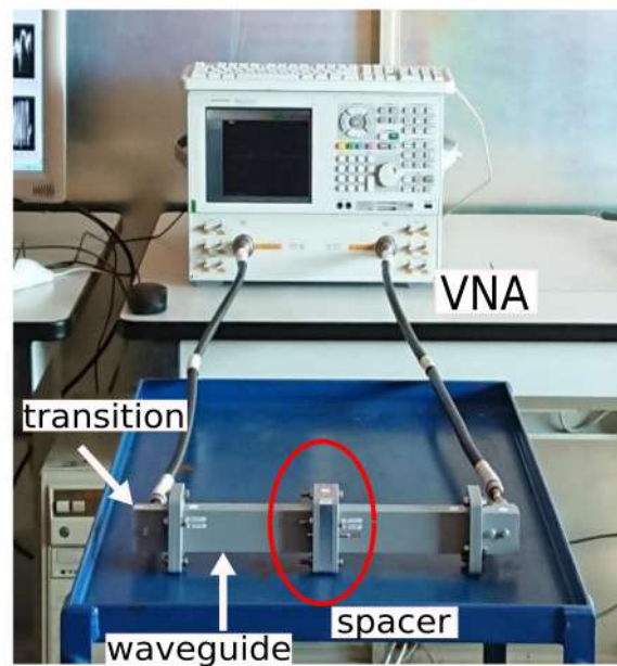
Figure 5. Scattering parameter measurement setup. The sample to be measured is inserted between the two waveguides [21], inside the spacer (red circle).
