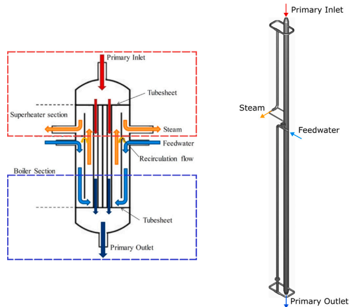
(a) OTSG conceptual scheme, highlighting the TOP and BOTTOM regions modelled in this work (red and blue boxes, respectively) [2].
