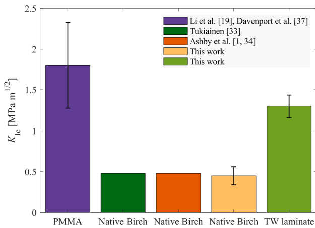
Fig. 4. Bar chart of fracture toughness data for different materials.
