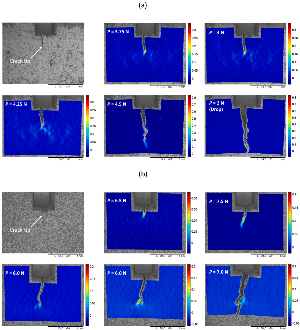
Fig. 9. Strain field \varepsilon_T : sequential images during the crack growth in (a) a native Birch sample and (b) a TW laminate. (unit: strain).
