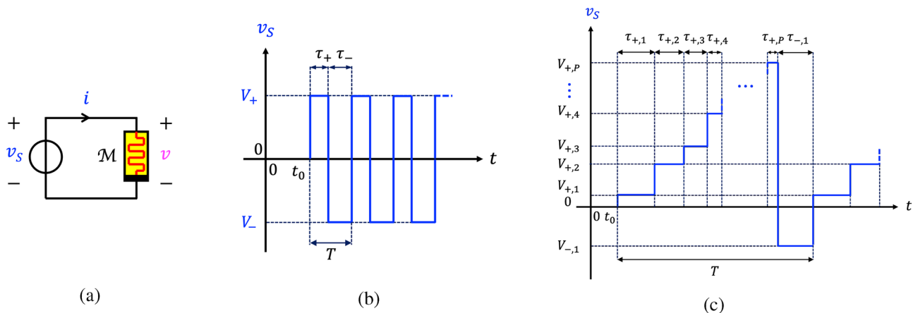
Figure 1. (a) Circuit employed to investigate the response of the \text{Ta}_2\text{O}_{5-x} ReRAM cell 15 to periodic square pulse-based voltage excitation signals. (b) Time course of a two-pulse-per-cycle train voltage stimulus. (c) Time waveform of a generalised pulse train voltage stimulus v_S , including P positive SET pulses and one negative RESET pulse per cycle. The RESET pulse of height V_- and width \tau_- follows the series of SET pulses. The i th SET pulse is V_{+,i} high and \tau_{+,i} wide, with i \in \{1, \dots, P\} . The ordering of the positive pulses from the lowest to the highest in each input cycle follows the convention adopted in the systematic methodology to engineer multistability in the steady-state oscillatory response of the ReRAM cell to a generalised train stimulus (refer to section “A systematic methodology to craft the pulse stimulus for enabling the ReRAM cell to support multiple oscillations around prescribed resistance levels”). However, this has no effect on the simulations. In fact, to facilitate their convergence, in the numerical investigations, discussed in section “Conclusions”, the SET pulses were listed from the most narrow to the most wide before being applied in this order one after the other across the device.
