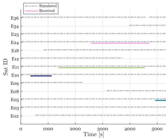
Figure 15: GAL E1BC satellites tracked during the scenario.
