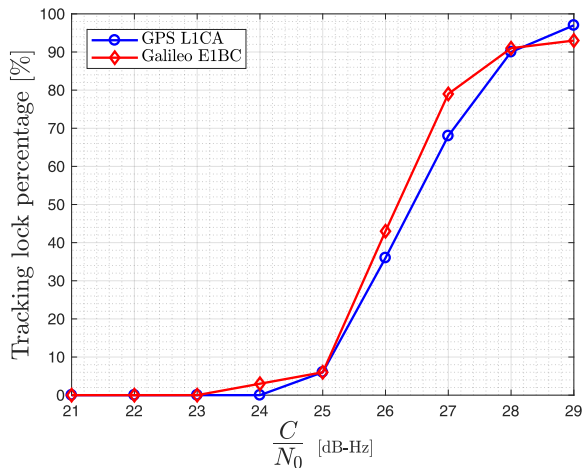
Figure 5: Tracking Lock Percentage over C/N0 before Optimization
