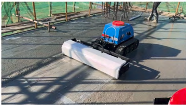
Fig. 15. Robot plastic film curing operation.
