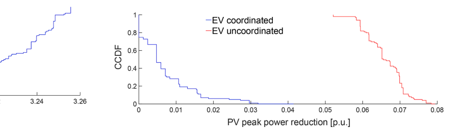
Fig. 19. PV peak power reduction in the sunny day.
