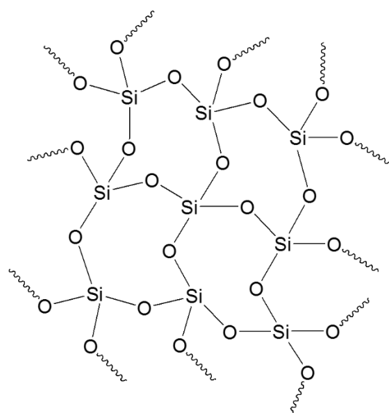
Figure 11. Three-dimensional network formed by subsequent condensation reactions.
