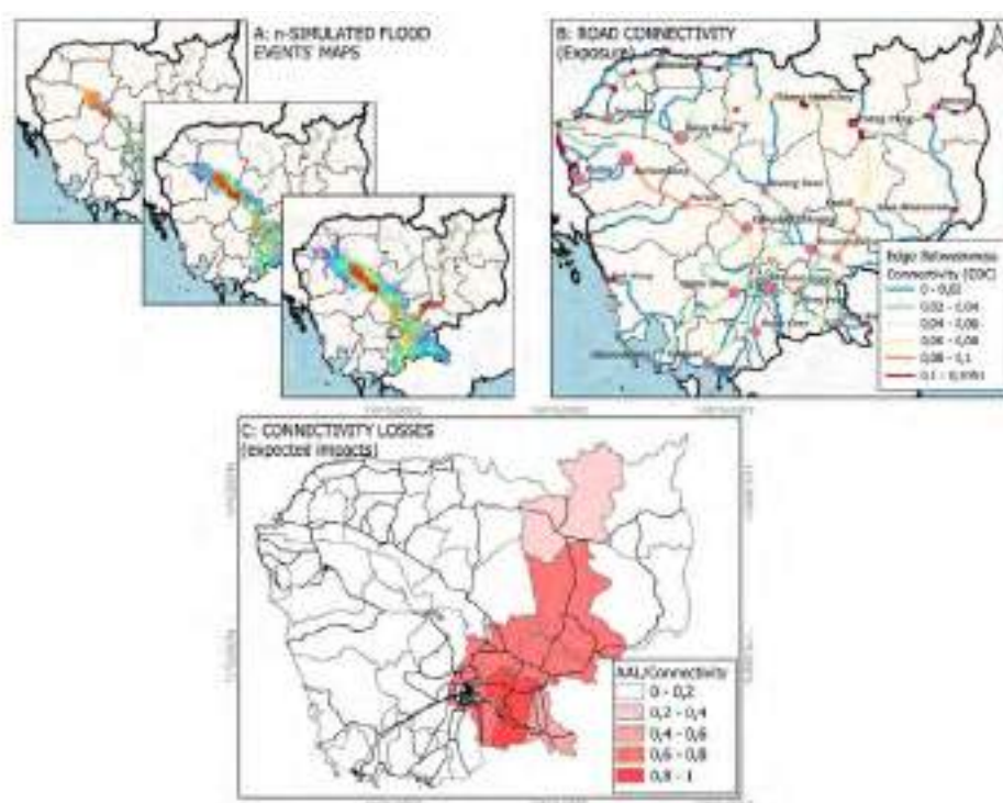
Figure 1 – Connectivity losses with a probabilistic approach. A) n -simulated flood events' maps; B) Road network classified by the edges' connectivity values, and potential origin (red dots)-destination (pink dots, service centers, main cities) pairs; C) Preliminary results showing administrative units classified by the ratio of AAL/total connectivity of road segments in each.
