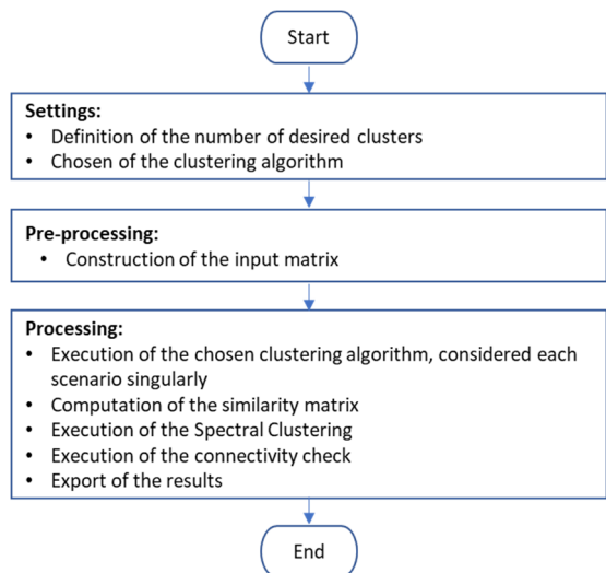
Fig. 3. Clustering algorithm.
