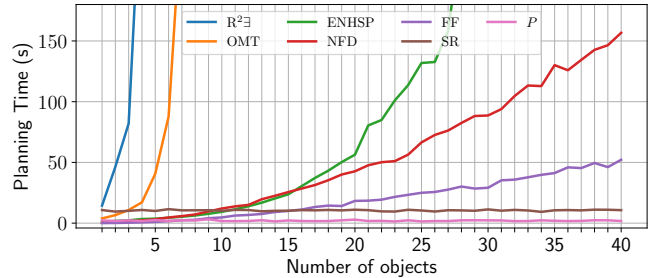
Figure 1: Performance on the LINEEXCHANGE domain.
