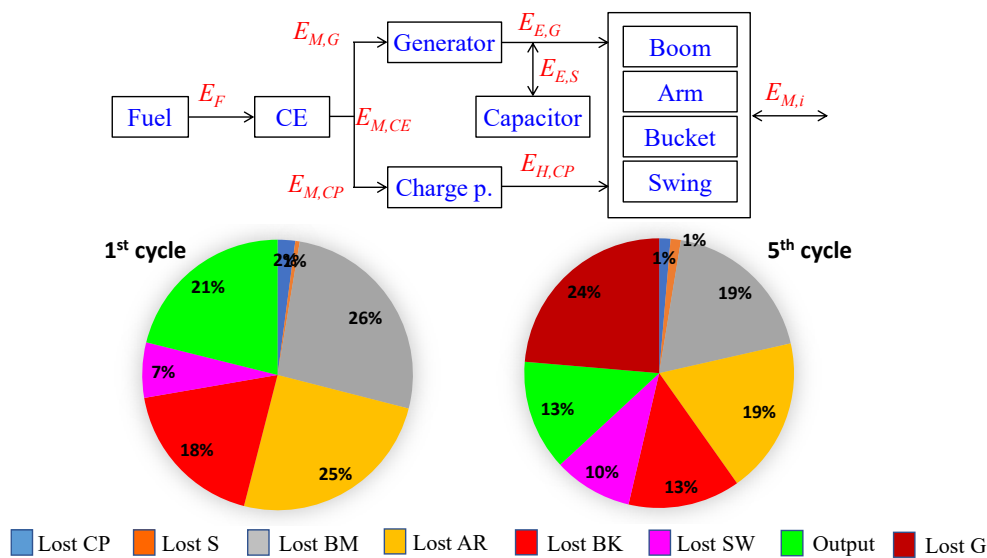
Figure 8. Block diagram of the energy flows inside the excavator and distribution of the losses.
