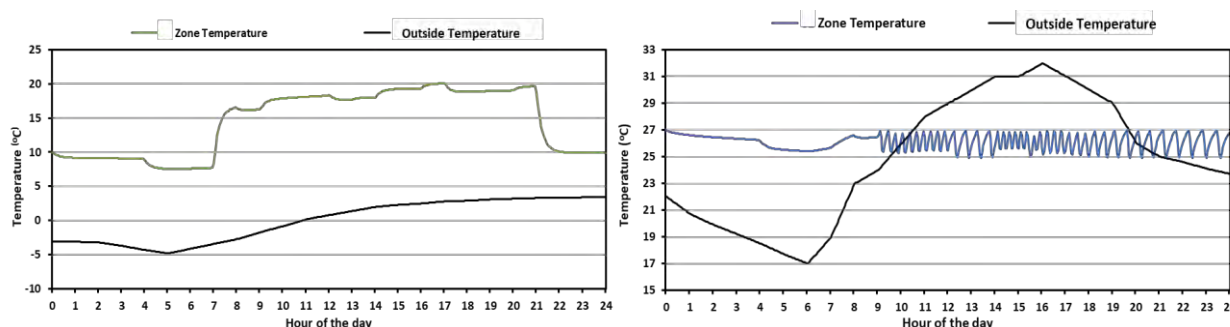
Figure 4. Zone temperature profiles: winter day (left) and summer day (right)
