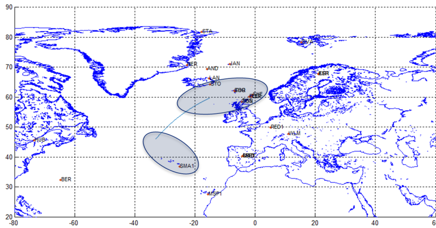
Fig. 15: Ground track respect to ground station locations, Isar LV orbit inclination of 68^\circ .
