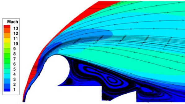
Fig. 20. Mach on a deformed shape (intermediate run).
