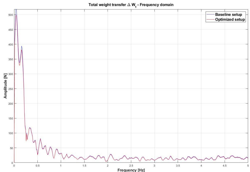
Figure 27. Comparison between the baseline provided setup and improved setup for the total weight transfer of the car in the frequency domain.
