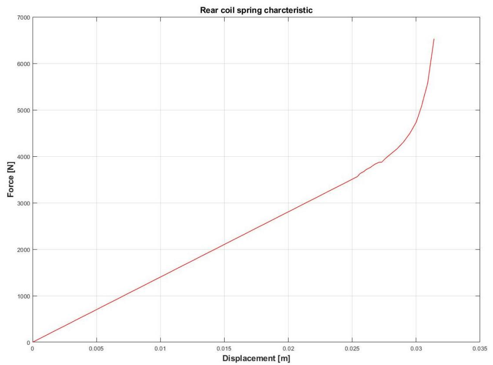
Figure 4. Rear coil spring characteristic.
