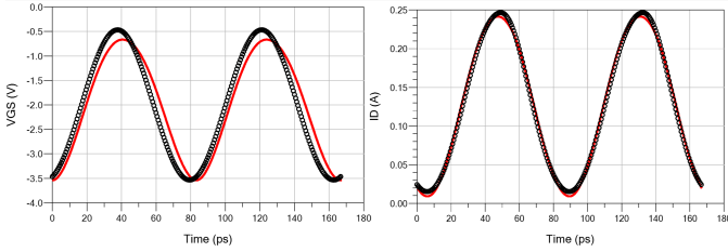
(b) Gate-source voltage and drain current waveforms.
