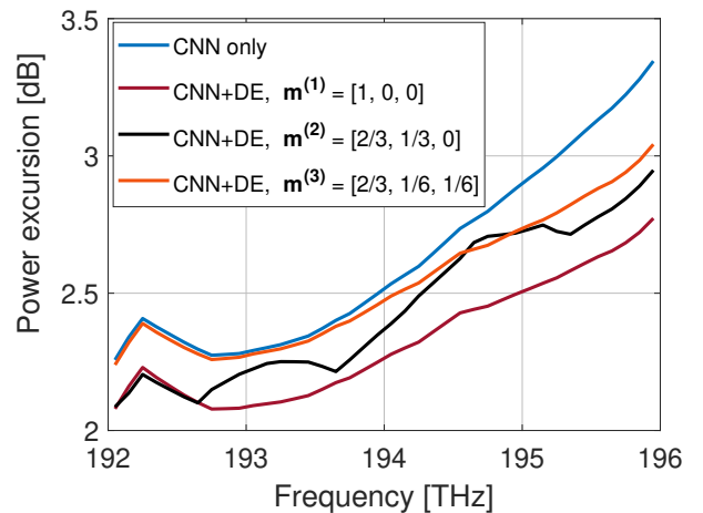
Fig. 6. Power excursion value computed as a function of frequency, shown for different pump power adjustment scenarios.
