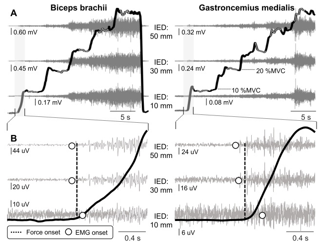
Fig. 1. Raw surface EMGs (grey traces) and torque data (black traces) are shown for the staircase, isometric contractions, separately for biceps brachii (BB) and Gastrocnemius medialis (GM) muscles. Data are shown for almost the whole trial in panel A, with bipolar EMGs obtained for 10 mm, 30 mm and 50 mm inter-electrode distances (IEDs) shown respectively from bottom to top. Note the different scales used to represent EMGs for different IEDs. An expanded portion of signals centered roughly at the torque onset (vertical, dashed line) is shown in B. EMG onsets computed for each IED (cf. Methods) are represented with white circles.
