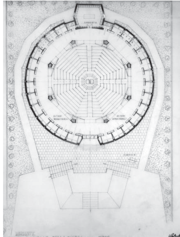
Fig. 01. Ido Avetta and Giulio Sciascia, competition design for the Domus Pacis chapel, Rome; first stage, October 1952 (ISACEM, GIAC, b. 885).
