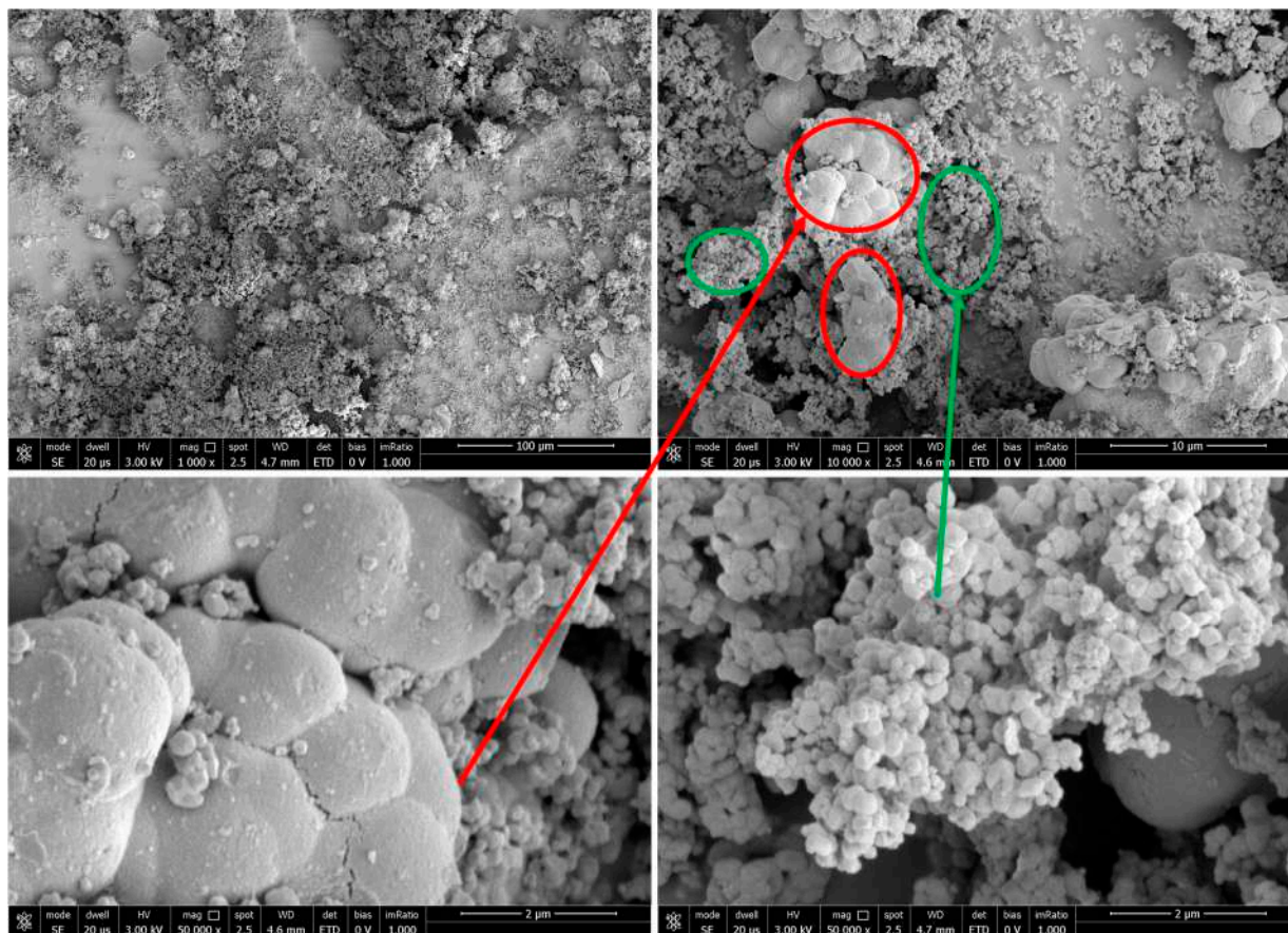
Figure 17. SEM micrographs at various magnifications of the Pd/CeO 2 -ZrO 2 catalytic system, regular spherical morphology circled in red and smaller average crystalline domain circled in green.
