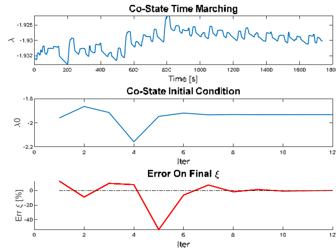
Figure 28. Co-State Identification results.
