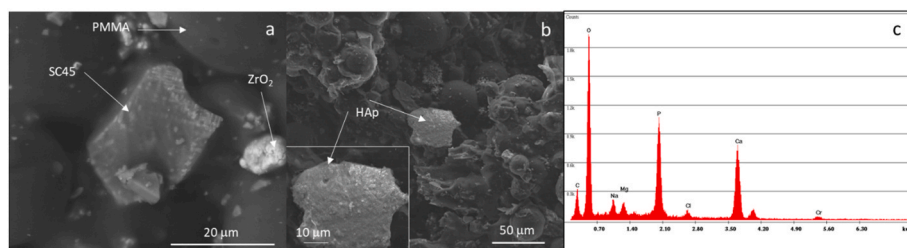
Fig. 2. P15 micrography (a) and SEM/EDS analysis of P15 after 4 weeks of soaking in SBF (b, c).
