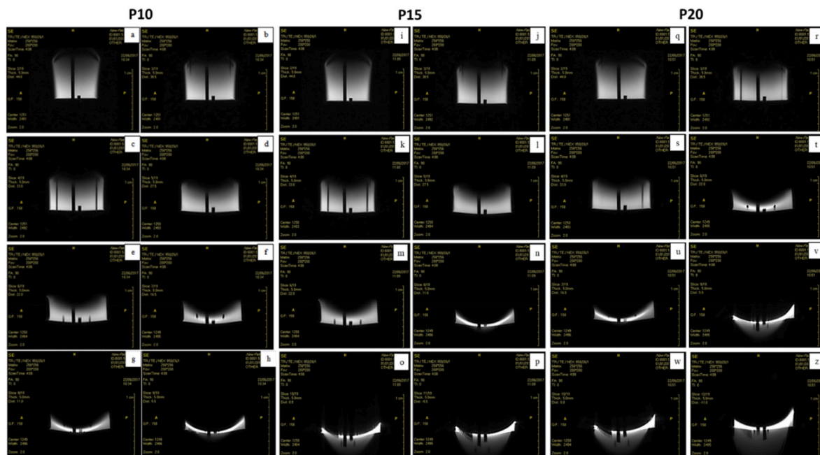
Fig. 11. Spin-echo scans of the phantom containing the contrast liquid and the composite bone cement samples weighted on T 1 , in different sections, from surface to the central one (P10: a-h; P15: i-p; P20: q-z).
