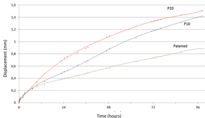
Fig. 8. Creep test (sample displacement vs. the time at 37 °C) for pure Palamed®, P10 and P20.
