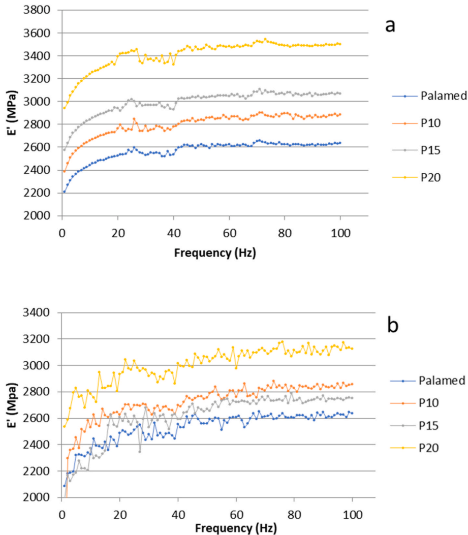
Fig. 6. Storage modulus E' evaluation by means of DMA at room temperature (a) and at 37 °C (b).
