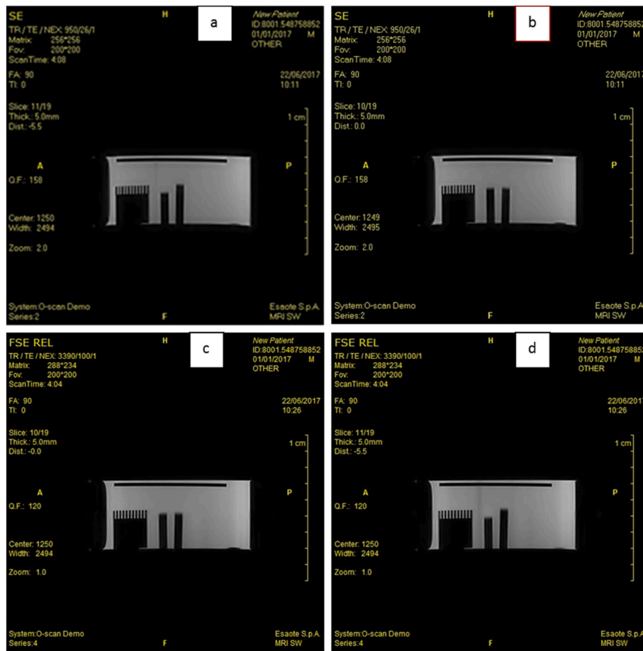
Fig. 10. Spin-echo scans of the phantom (central sections) containing the contrast liquid and the plain Palamed® samples weighted on T 1 (a, b) and T 2 (c, d).
