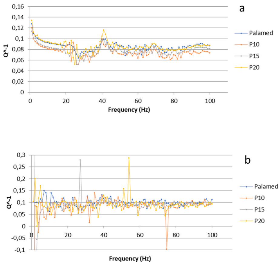
Fig. 7. Loss factor at room temperature (a) and at 37 °C (b).
