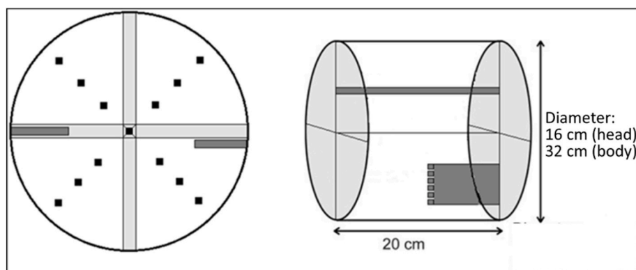
Fig. 1. Schematic view of the cylindrical phantom with reference rigid structures.
