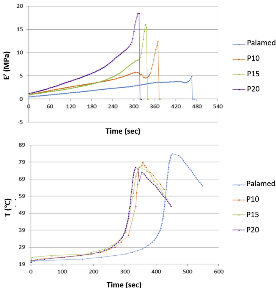
Fig. 4. Elastic modulus (a) and temperature (b) trends vs time obtained by means of dynamo-mechanical analysis.
