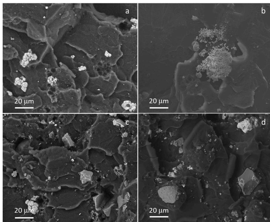
Fig. 5. Micrography of the fracture surfaces of plain Palamed® (a, b) and P10 composite bone cement (c, d) after three points bending test at room temperature [16] (b, d) and 37 °C (a, c).
