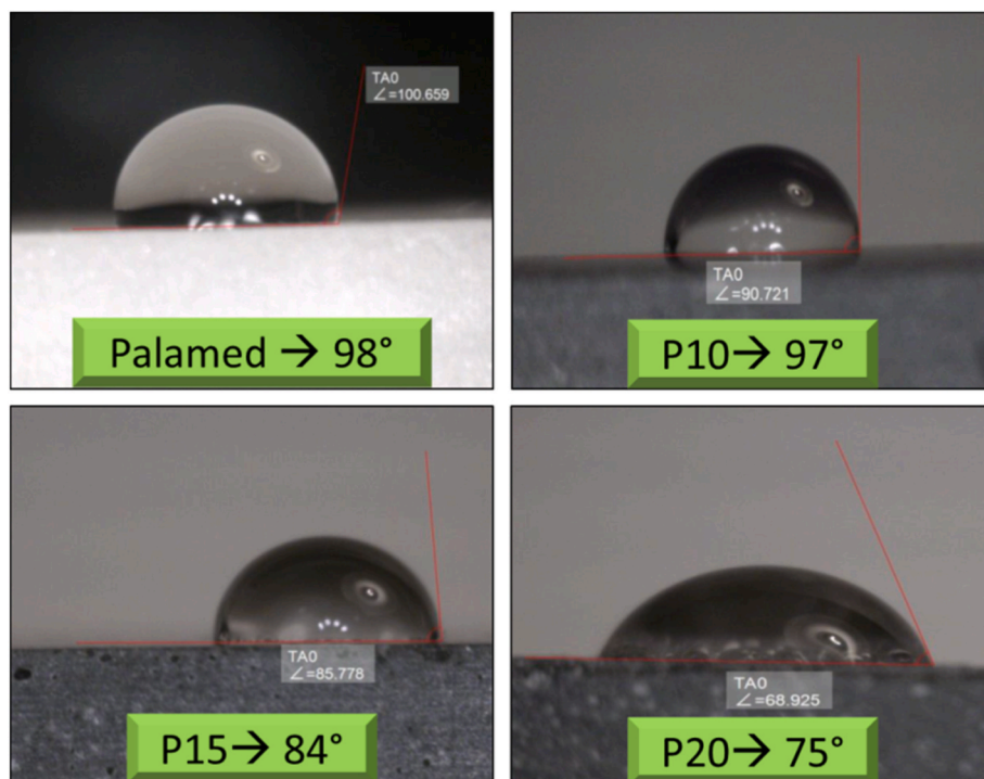
Fig. 3. Analysis of wettability.
