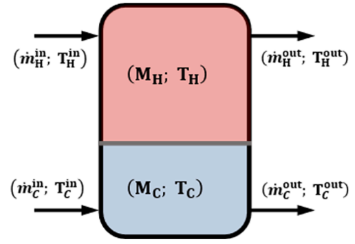
Fig. 6. Schematic of the thermal storage according to the model adopted in the analysis.
