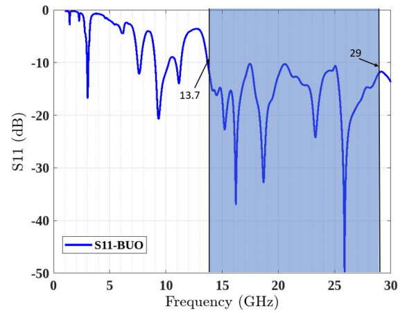
Fig. 6. S_{11} for MIMO through BUO
