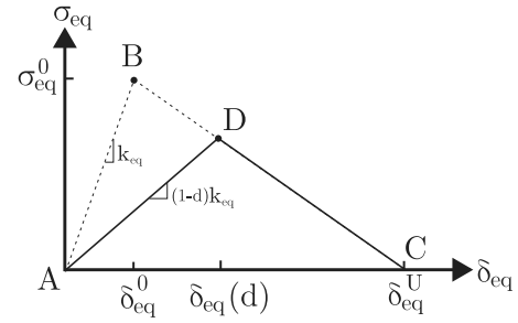
Fig. 3. Constitutive relation for the equivalent stress and displacement.
