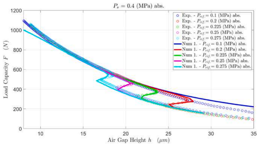
Fig. 20. Comparison between the experimental and numerical load capacity curves obtained at P_s=0.4 absolute MPa and different reference pressures P_{rif}=0.1, 0.2, 0.225, 0.25, 0.275 absolute MPa.
