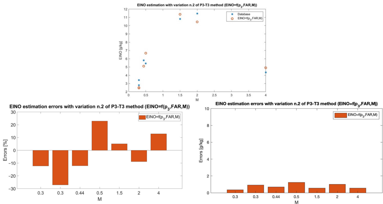
Figure 11. Comparison of EINO predictions with the new formulation in Equation (9) and emission estimations from 0D chemical-kinetic simulations ( top ) and related relative and absolute errors ( bottom ).
