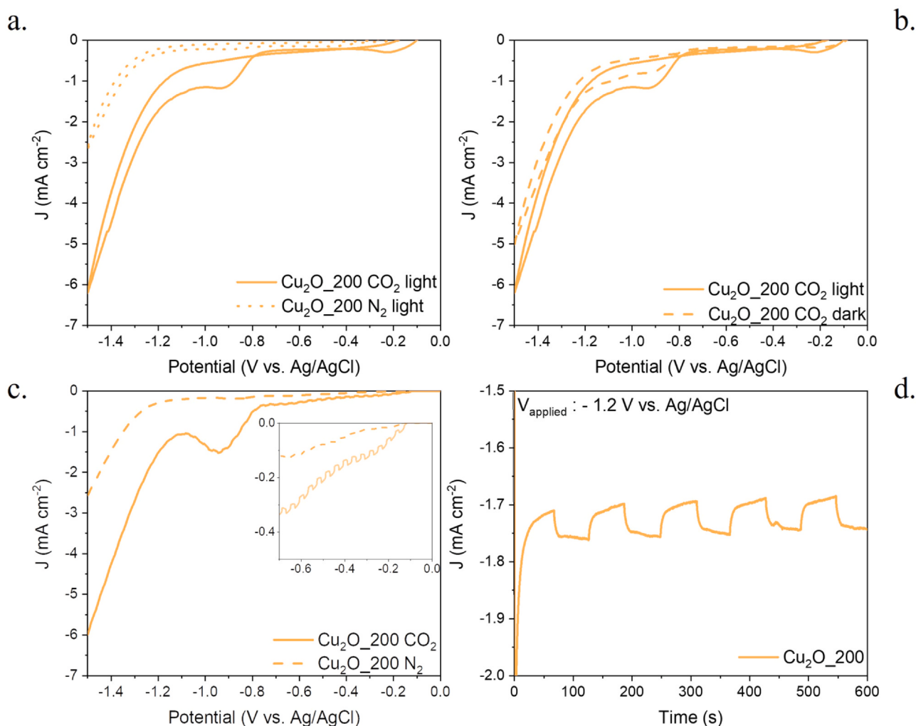
Fig. 8 – Results of PEC tests of \text{Cu}_2\text{O}_{200} sample, in particular: (a) comparison of CVs carried out in \text{N}_2 and \text{CO}_2 saturated environment under illumination, (b) comparison of CVs carried out in \text{CO}_2 saturated environment both in dark and light conditions, (c) LSVs tests carried out in \text{N}_2 and \text{CO}_2 saturated environment, with chopped illumination (each 2 s), and (d) chronoamperometry test 10 min lasting with an applied potential of -1.2 V vs. Ag/AgCl, under chopped light each 1 min.
