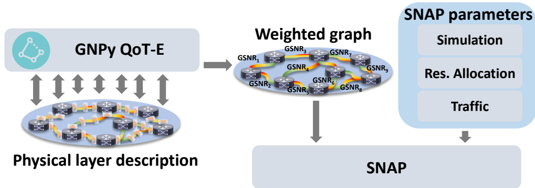
Fig. 2.8 SNAP workflow.
