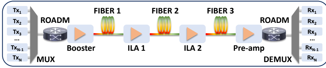
Fig. 2.1 Illustration of an OLS and its main components.
