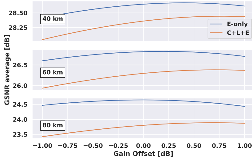
Fig. 4.3 Average E-band GSNR dependency on BDFA gain offset in a single span OLS for 40, 60 and 80 km with E-band only and C+L+E-band transmission.
