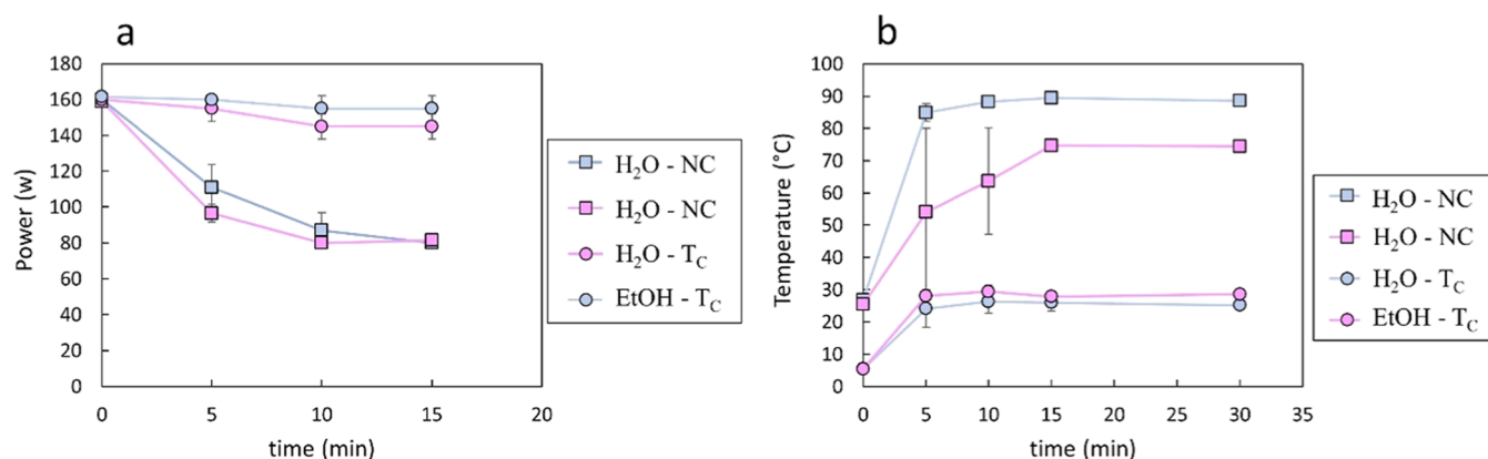
Figure 3. Applied power (a) and temperature profile (b) measured during the sonication tests performed with H 2 O and ethanol (EtOH) as solvents, with (T C ) and without (NC) temperature control.
