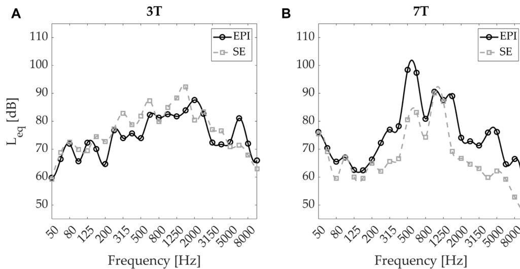
FIGURE 8 Noise Measurements with a head phantom: EPI and SE sequences evaluated as equivalent sound pressure level in one-third octave bands for (A) 3 T and (B) 7 T scanners at the left ear isocenter position.
