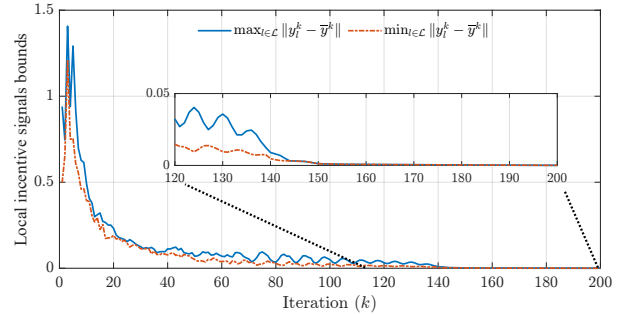
Fig. 2. Consensus of the local incentive signals.
