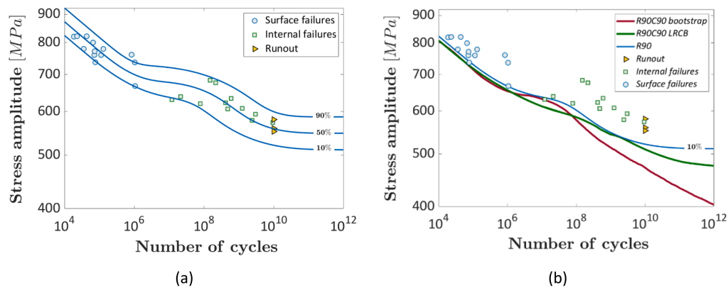
Fig. 9. validation of the duplex P-S-N design curves for datasets showing a duplex in the LCF-VHCF life range: a) median, 0.1-th and 0.9-th quantile P-S-N curves; b) 0.1-th and design P-S-N curves estimated with the LRCB and the bootstrap approach.
