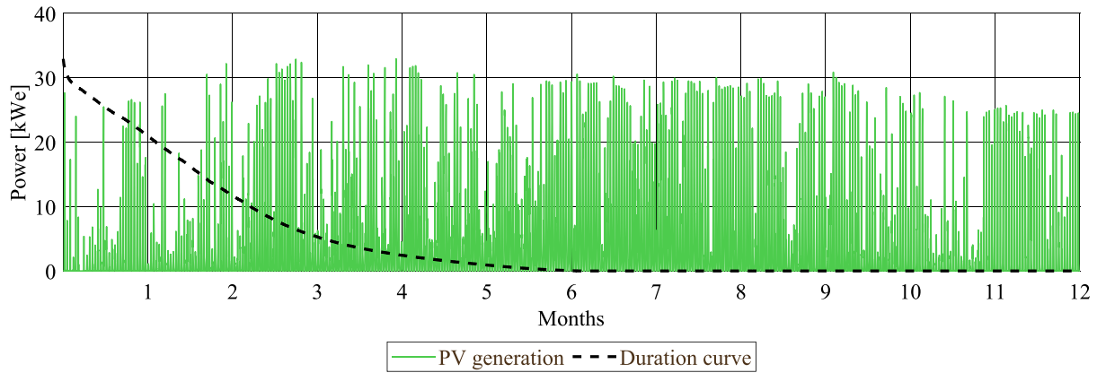
Fig. 5. Annual profile of PV production and its duration curve (data are taken from [43]).
