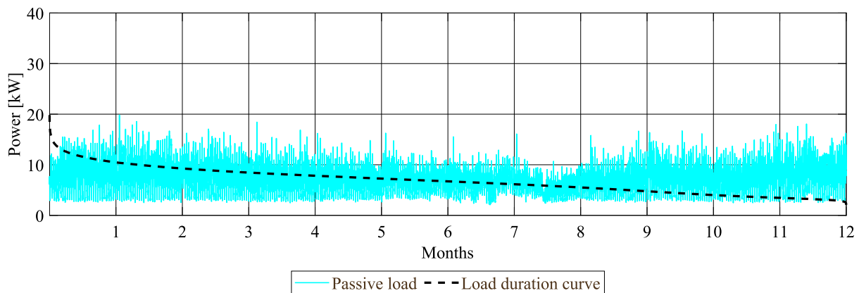
Fig. 4. Annual profile of the passive electricity load and its load duration curve (this profile does not include the electricity consumption of the LP2H units).
