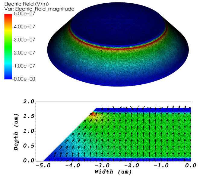
Fig. 3: Electric field profile computed with FBMC3D at 35V. Top panel shows the electric field on the 3-D device. Bottom panel shows a cross-section of the 3-D device with electric field vectors.
