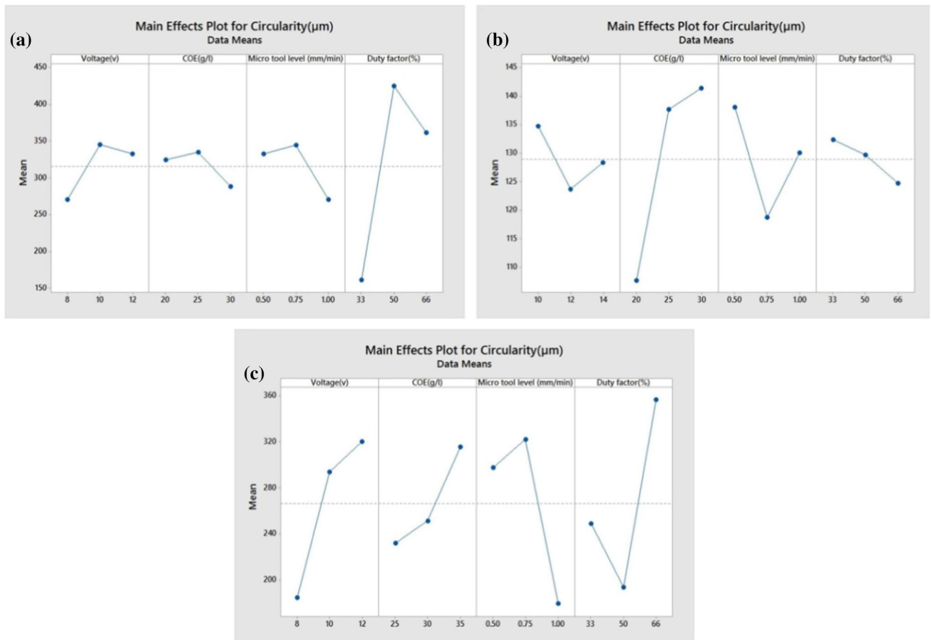
Fig. 7 Influence of machining factors on circularity while machining with a NaCl, b NaNO 3 and c hybrid electrolyte
