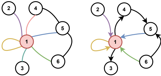
FIGURE 2. Undirected (left) and a directed (right) graph representation. The neighbourhood of node 1 is highlighted through coloured edges in both graphs. For the undirected graph, the neighbourhood is composed by the nodes that are connected to node 1 : node 2, node 3, node 4, node 5, node 6. Instead, for the directed one, the neighbourhood is composed only by the nodes that have incoming edges to node 1: node 2, node 5, node 6. It is worth mentioning that in some cases graphs may also have edges starting and ending on the same node (self-loop), which may be relevant for some graph convolution formalisation.
