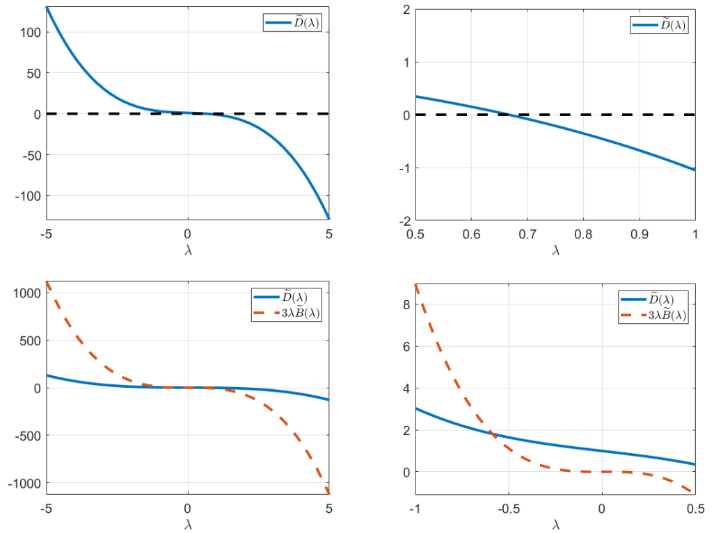
Figure 7. (Top, Left): Graph of \tilde{D} (blue line) as a cubic function of \lambda . (Bottom, Left): Graphs of \tilde{D} (blue line) and 3\lambda\tilde{B}(\lambda) (orange line). (Right): zoom of the left panels.
