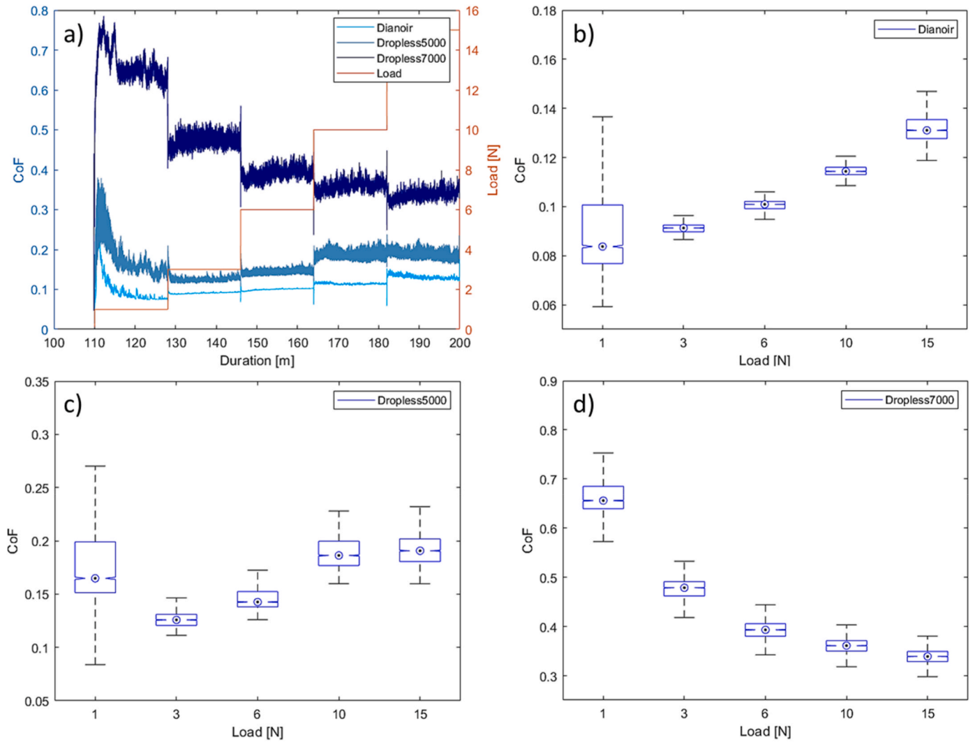
Fig. 19. (a) Rough friction curve recorded for Friction test An under increasing load and a constant speed of 0.1 m/s (b–d) Summary statistic box plots for Dianoir, Dropleless5000, and Dropleless7000, respectively. The blue dot inside each box represents the median value of the load level. Each loading step lasted 3 min. (For interpretation of the references to colour in this figure legend, the reader is referred to the Web version of this article.)
