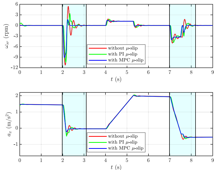
Fig. 4. Simulation Test: performance comparison with MPC micro-slip (blue), PI micro-slip (green) and without micro-slip (red). Top plot: Slipping speed \omega_{sr} . Bottom plot: Longitudinal acceleration a_x . (For interpretation of the references to colour in this figure legend, the reader is referred to the web version of this article.)
