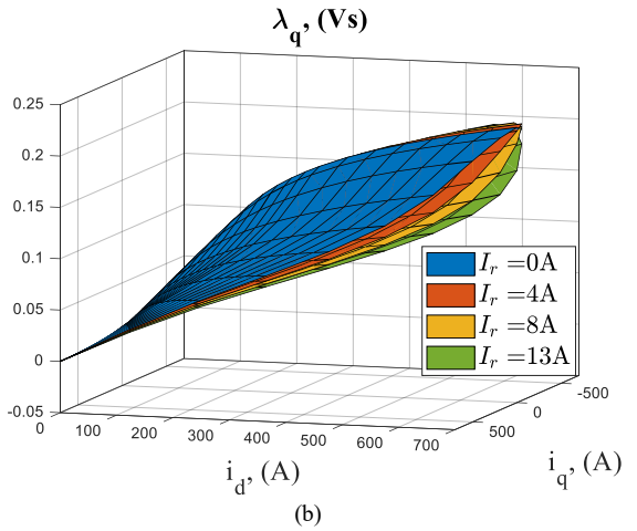
Fig. 7 Current-to-flux linkage model for the WFSM considered for the sizing code validation.
