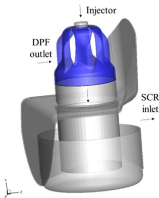
Fig. 3 UWS mixing subsystem for geometry B
